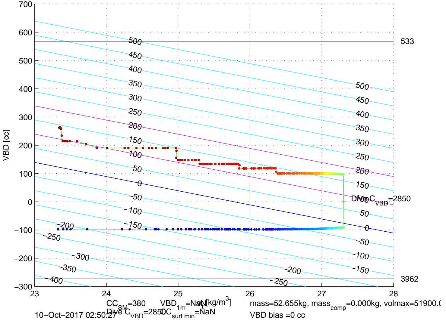
p6350647: SG635 Mission 7 Jul 2017 10-Oct-2017 02:08:52Z – buoyancy contoured
