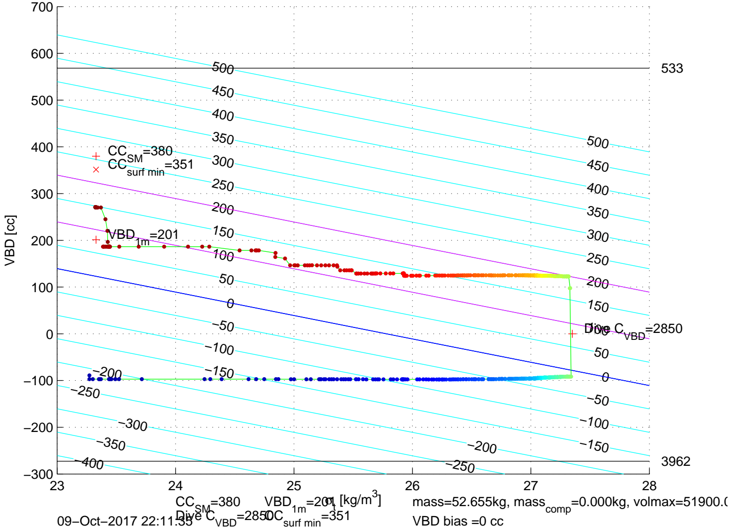
p6350646: SG635 Mission 7 Jul 2017 09–Oct–2017 21:44:43Z – buoyancy contoured
