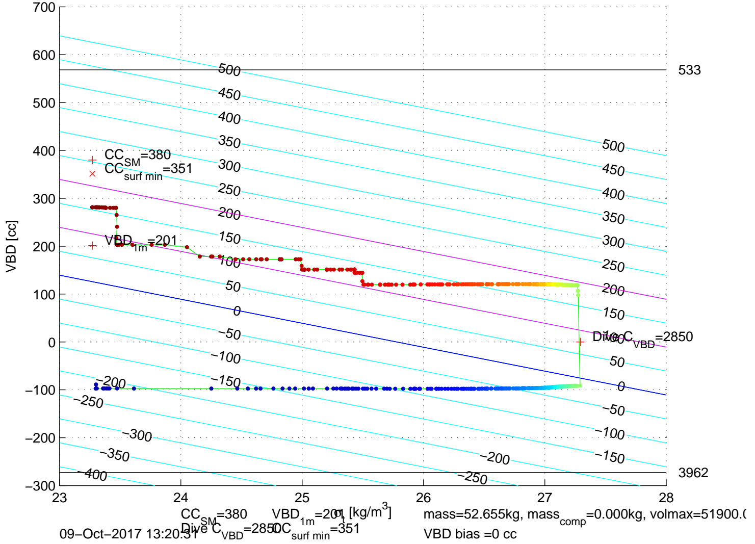
p6350644: SG635 Mission 7 Jul 2017 09–Oct–2017 12:48:45Z – buoyancy contoured
