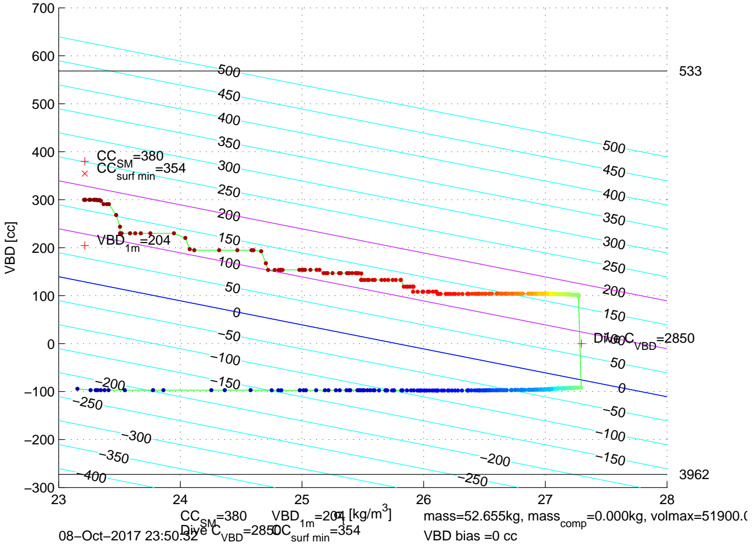
p6350641: SG635 Mission 7 Jul 2017 08–Oct–2017 23:21:04Z – buoyancy contoured
