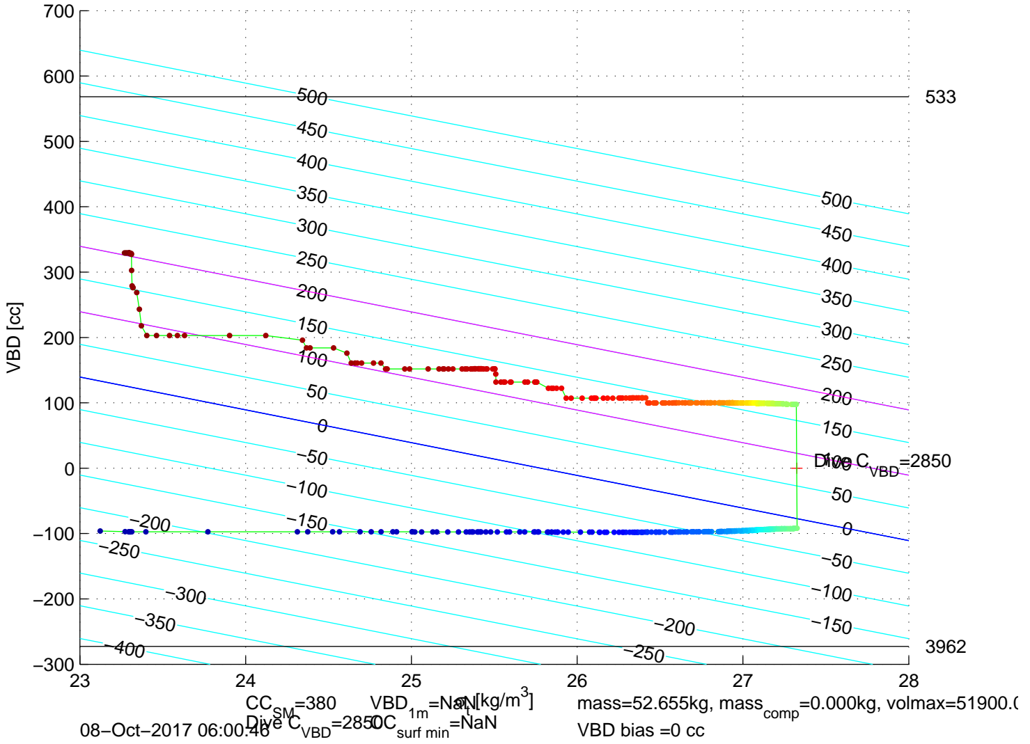
p6350637: SG635 Mission 7 Jul 2017 08-Oct-2017 05:31:36Z – buoyancy contoured
