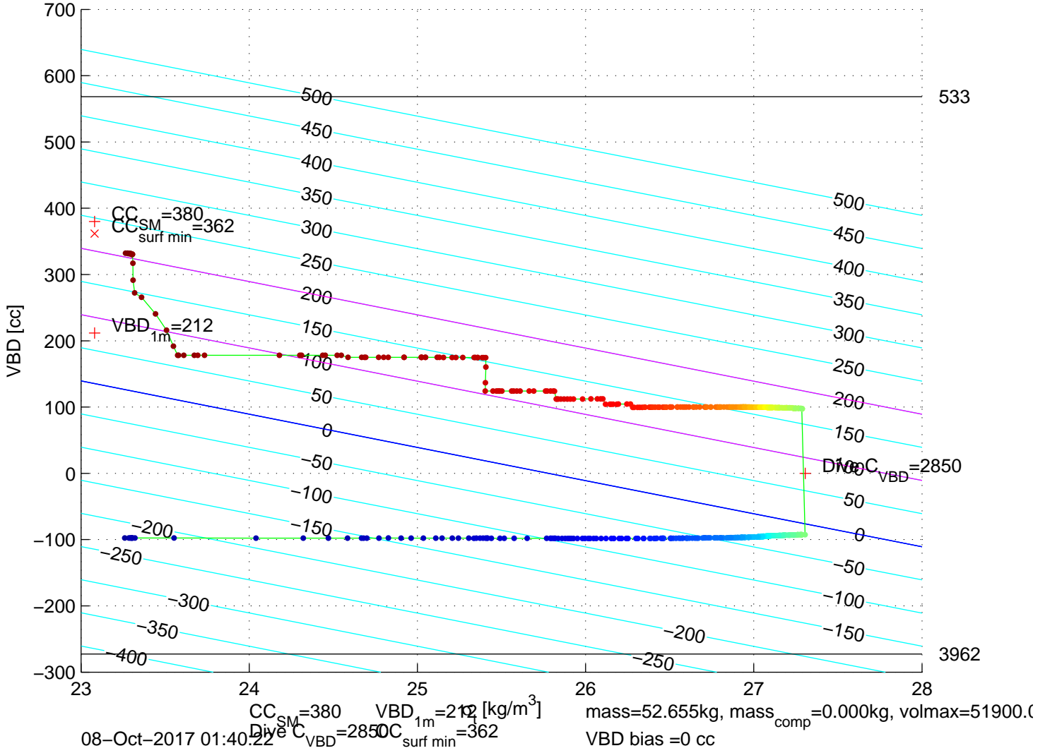
p6350636: SG635 Mission 7 Jul 2017 08–Oct–2017 01:00:05Z – buoyancy contoured
