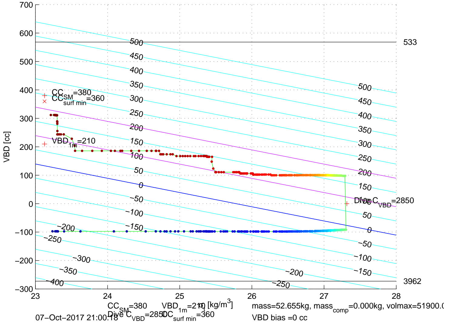
p6350635: SG635 Mission 7 Jul 2017 07–Oct–2017 20:26:32Z – buoyancy contoured
