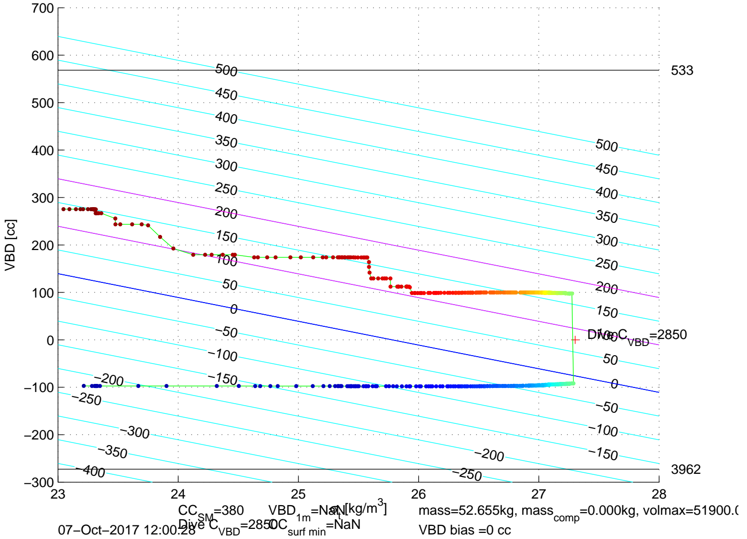
p6350633: SG635 Mission 7 Jul 2017 07–Oct–2017 11:27:47Z – buoyancy contoured
