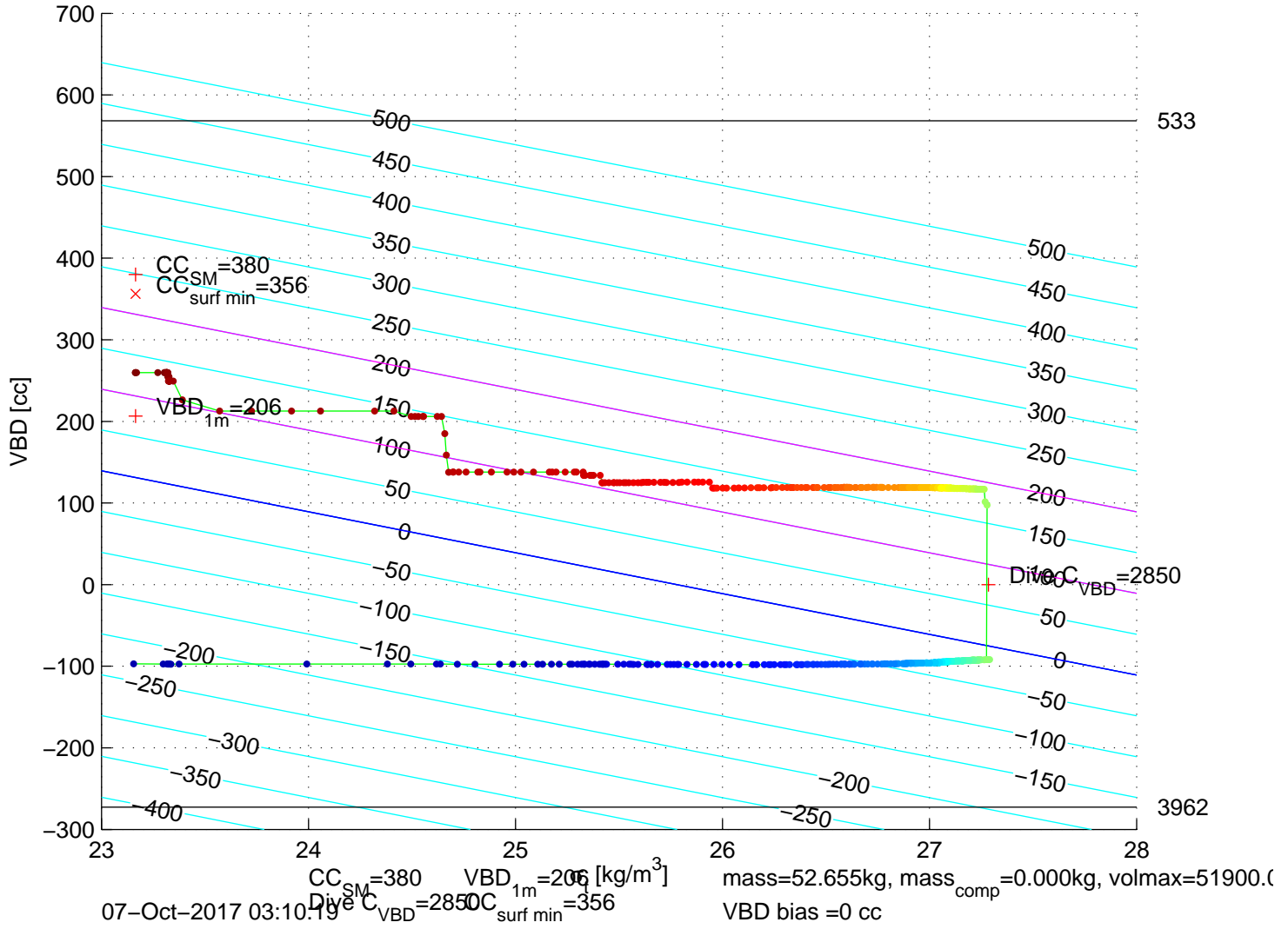
p6350631: SG635 Mission 7 Jul 2017 07-Oct-2017 02:41:03Z – buoyancy contoured
