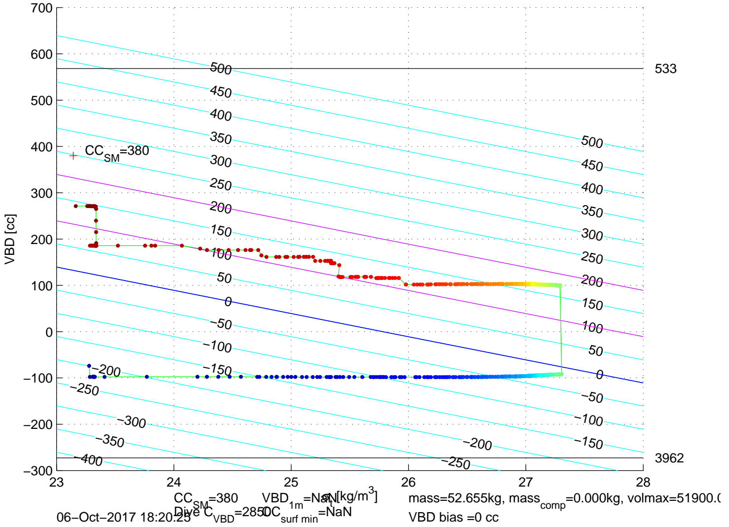
p6350629: SG635 Mission 7 Jul 2017 06–Oct–2017 17:38:02Z – buoyancy contoured
