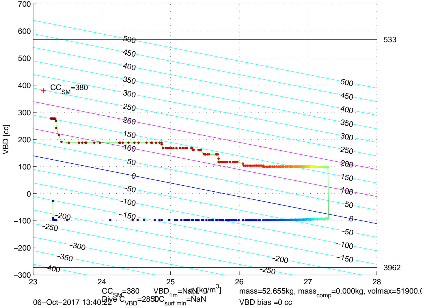
p6350628: SG635 Mission 7 Jul 2017 06–Oct–2017 13:05:27Z – buoyancy contoured
