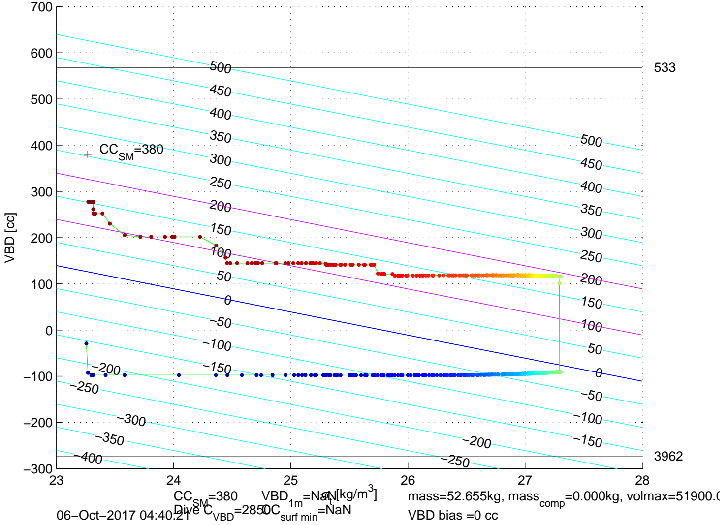
p6350626: SG635 Mission 7 Jul 2017 06–Oct–2017 04:09:48Z – buoyancy contoured
