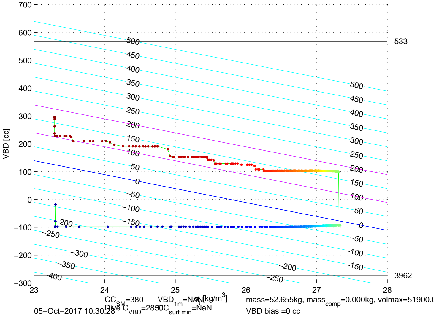
p6350622: SG635 Mission 7 Jul 2017 05–Oct–2017 09:54:57Z – buoyancy contoured
