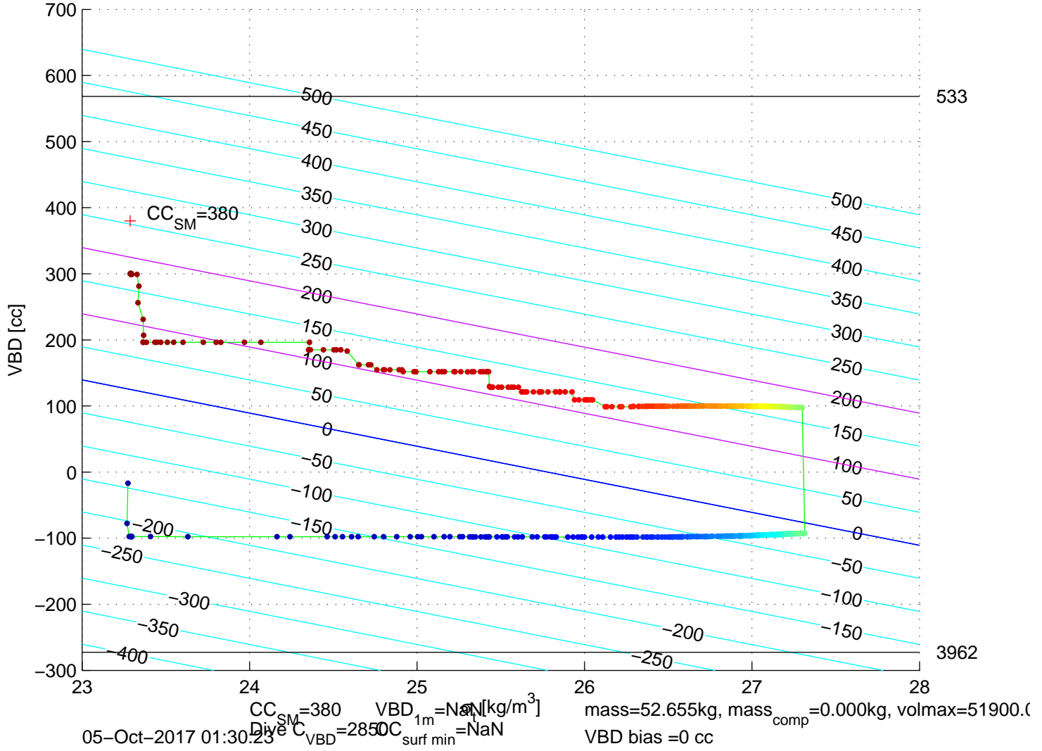
p6350620: SG635 Mission 7 Jul 2017 05–Oct–2017 00:50:42Z – buoyancy contoured
