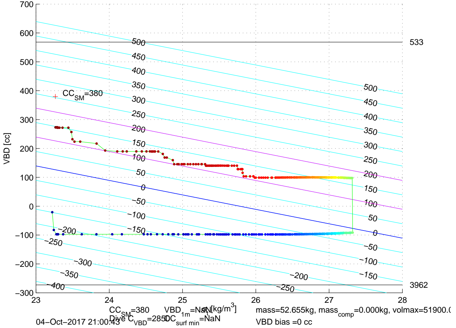
p6350619: SG635 Mission 7 Jul 2017 04–Oct–2017 20:17:16Z – buoyancy contoured
