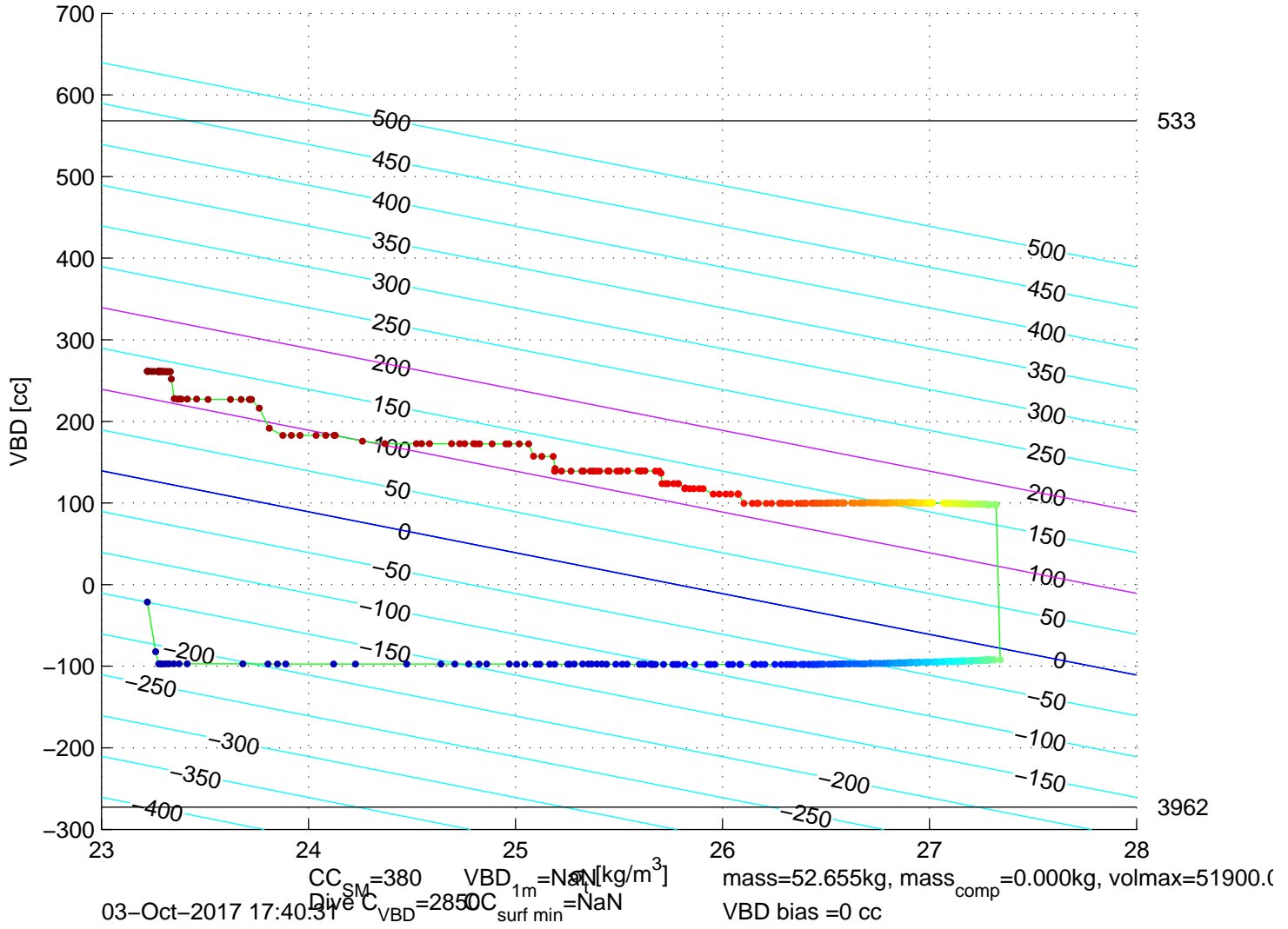
p6350613: SG635 Mission 7 Jul 2017 03–Oct–2017 17:10:27Z – buoyancy contoured
