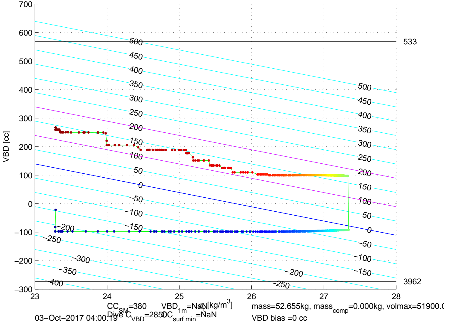
p6350610: SG635 Mission 7 Jul 2017 03–Oct–2017 03:10:06Z – buoyancy contoured
