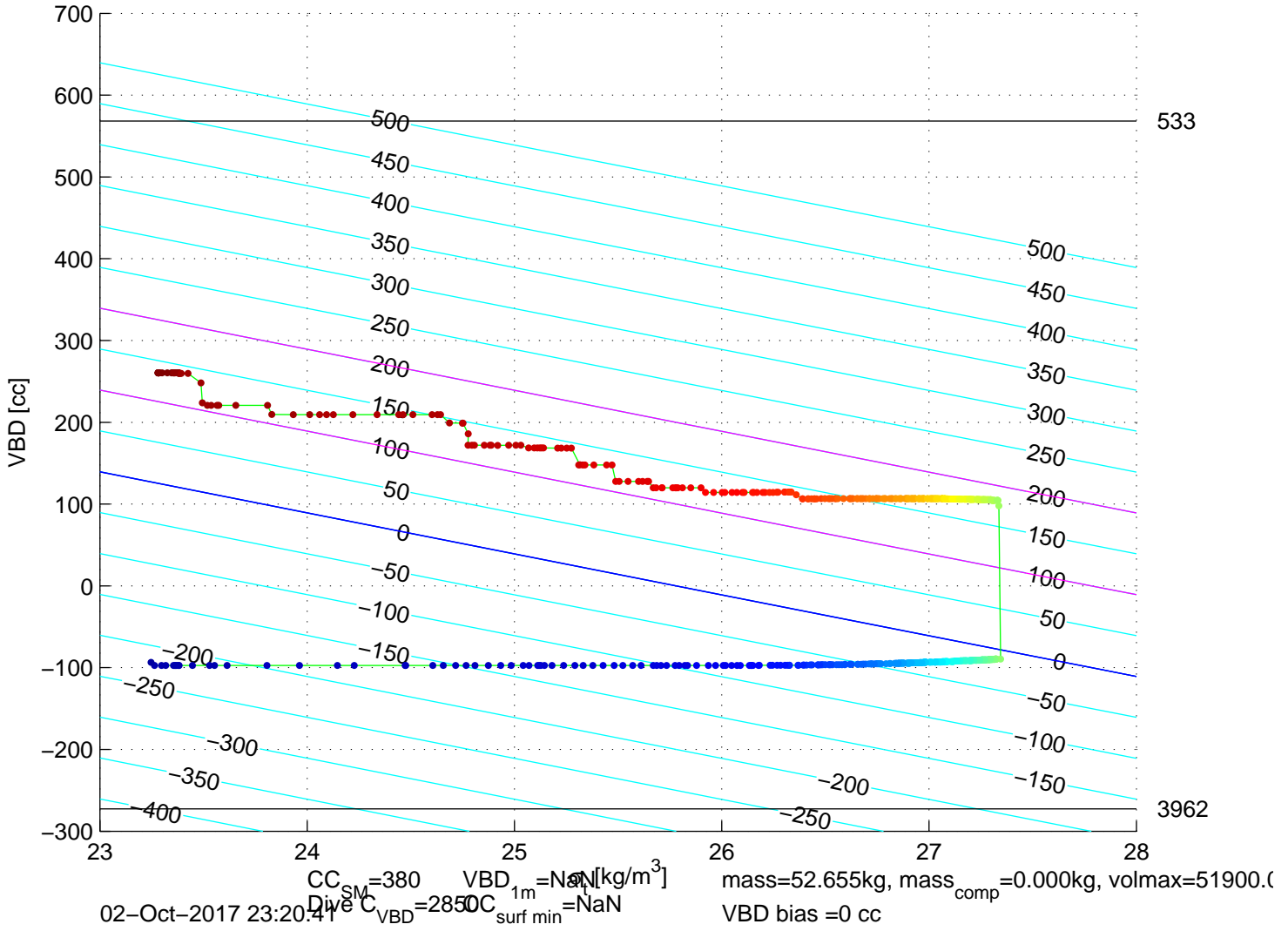
p6350609: SG635 Mission 7 Jul 2017 02–Oct–2017 22:35:30Z – buoyancy contoured
