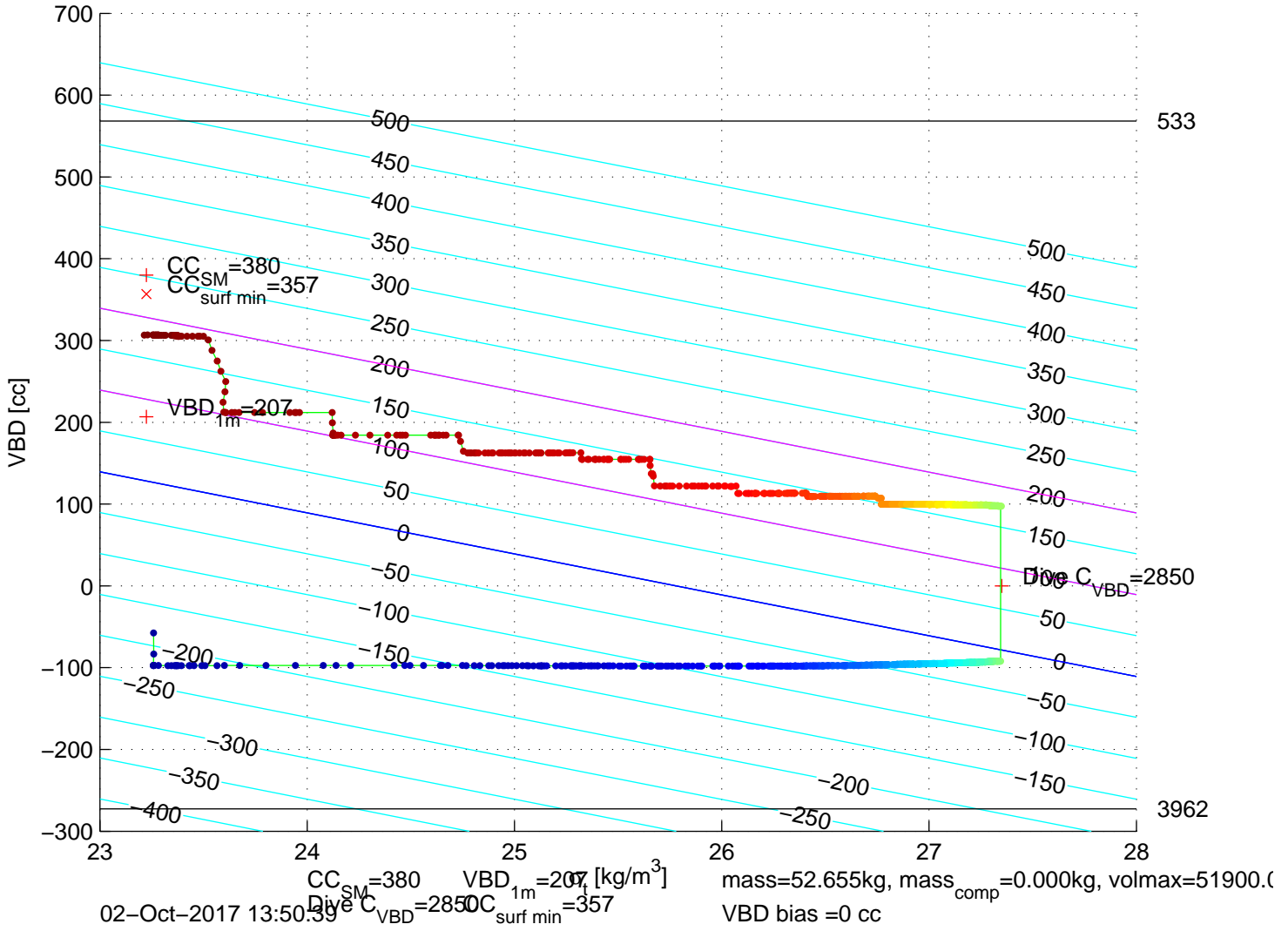
p6350607: SG635 Mission 7 Jul 2017 02–Oct–2017 12:53:51Z – buoyancy contoured
