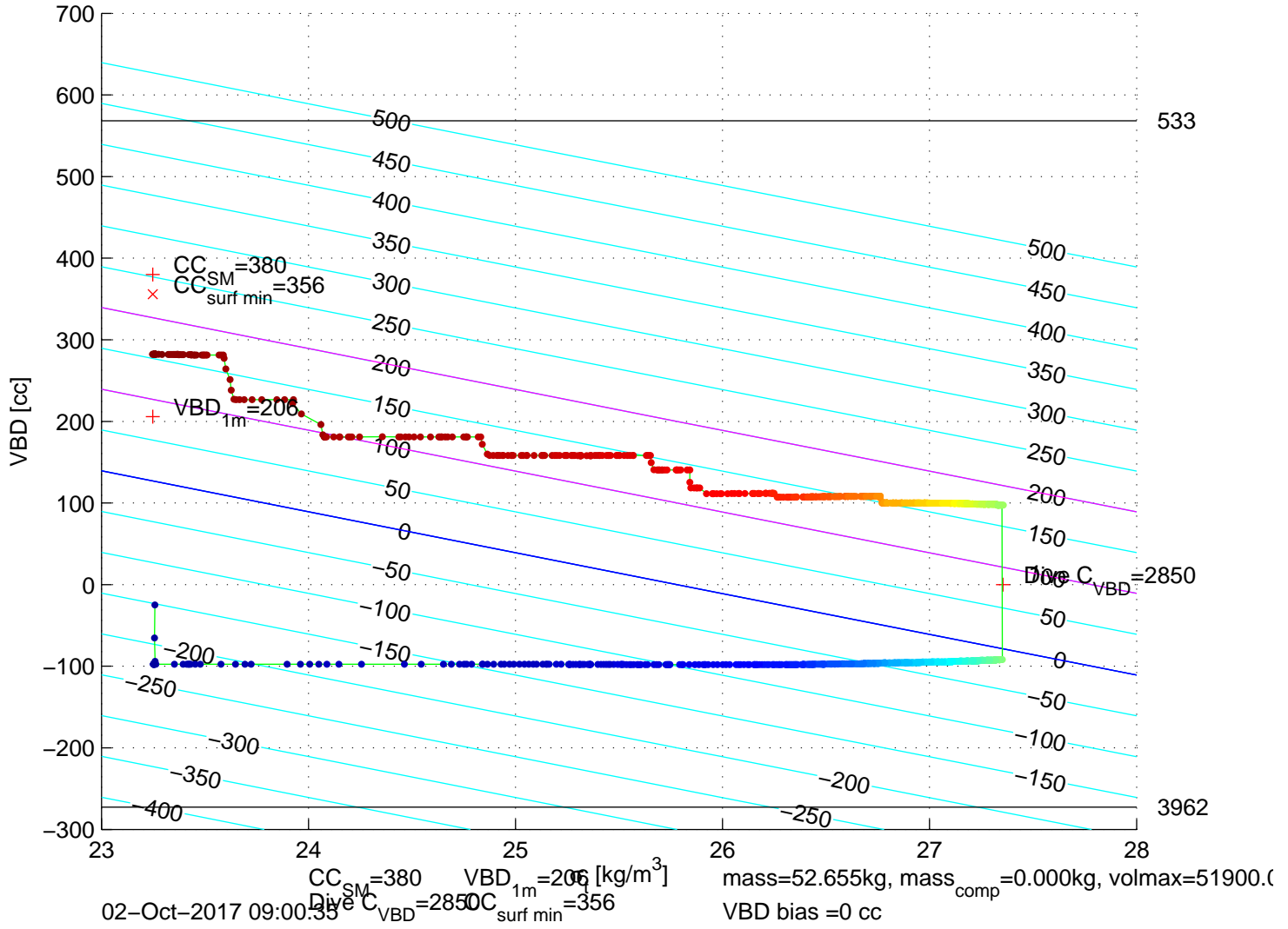
p6350606: SG635 Mission 7 Jul 2017 02–Oct–2017 08:07:17Z – buoyancy contoured
