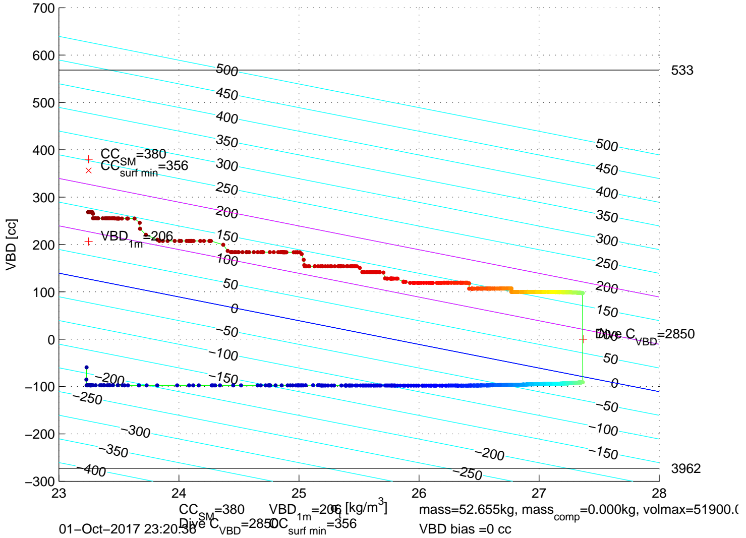
p6350604: SG635 Mission 7 Jul 2017 01–Oct–2017 22:25:51Z – buoyancy contoured
