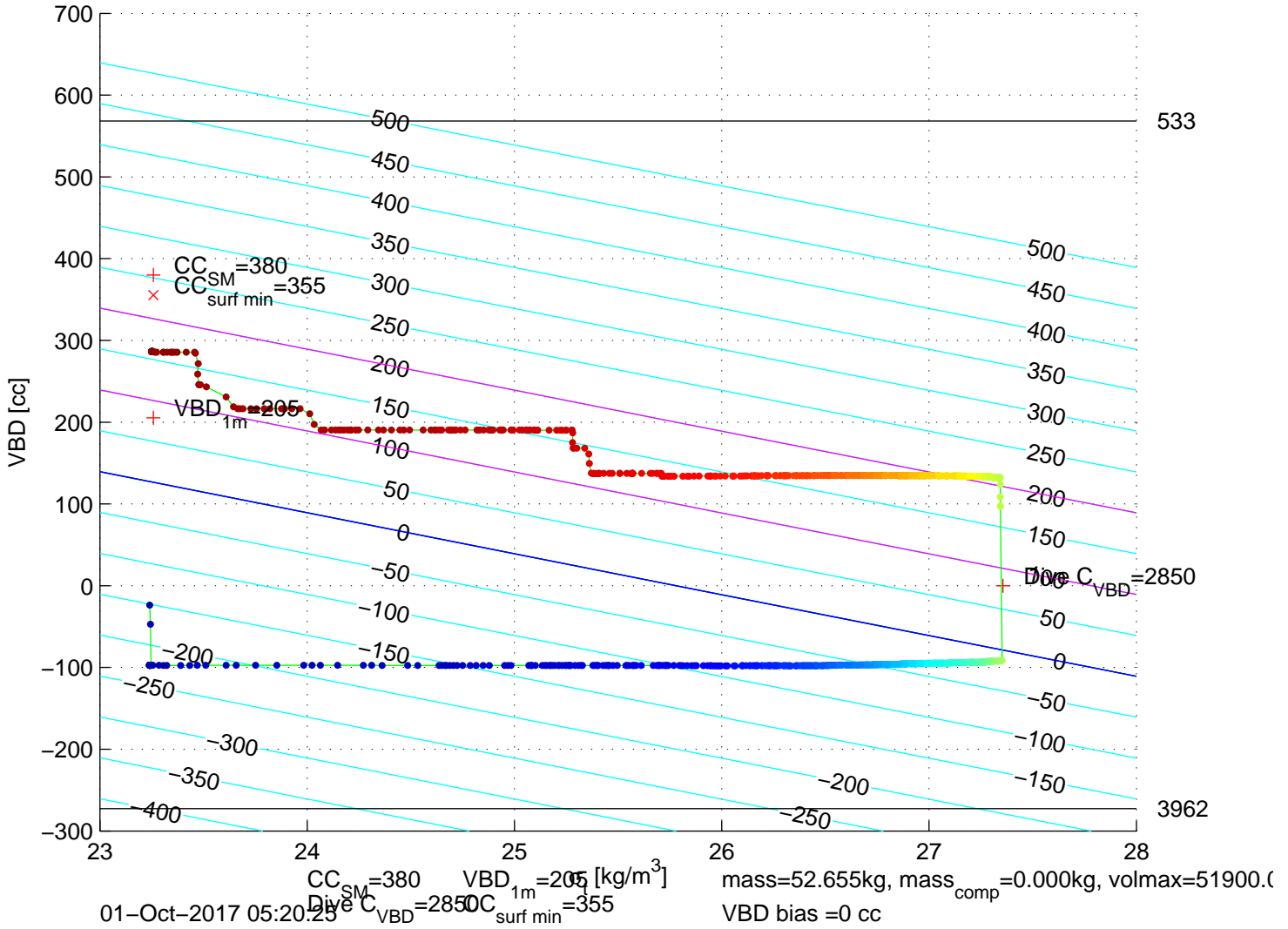
p6350600: SG635 Mission 7 Jul 2017 01-Oct-2017 04:52:49Z – buoyancy contoured
