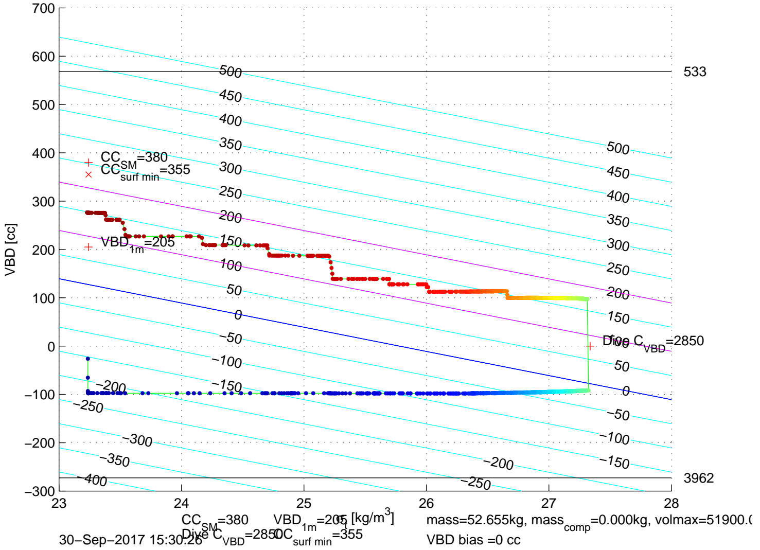
p6350597: SG635 Mission 7 Jul 2017 30-Sep-2017 14:46:43Z – buoyancy contoured
