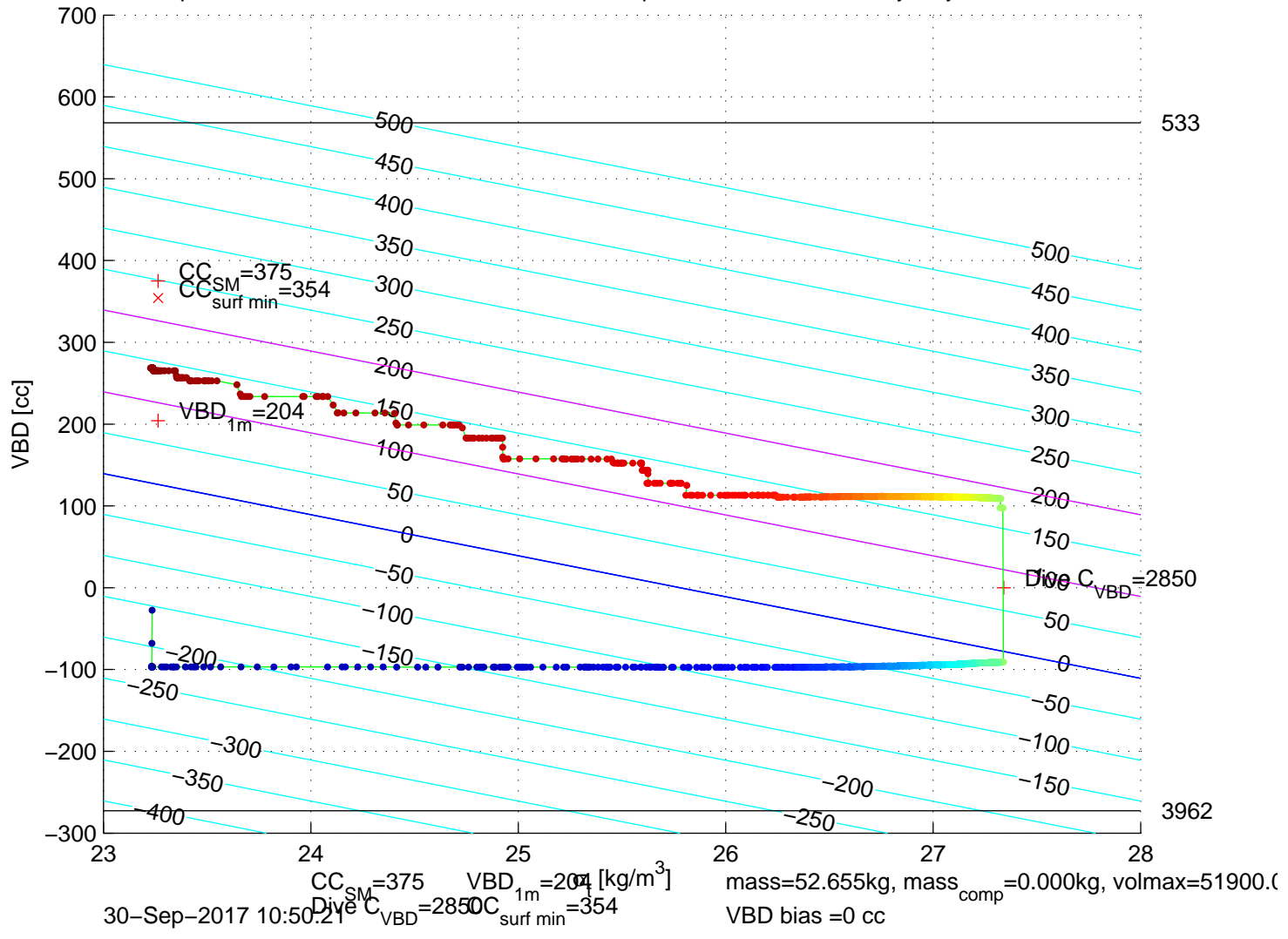
p6350596: SG635 Mission 7 Jul 2017 30-Sep-2017 10:05:05Z – buoyancy contoured
