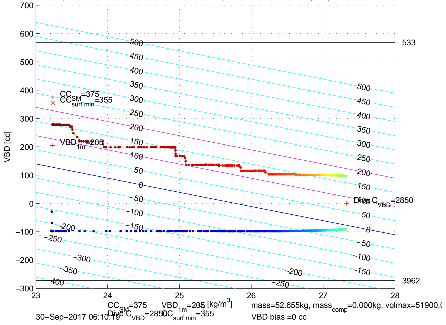
p6350595: SG635 Mission 7 Jul 2017 30-Sep-2017 05:19:42Z – buoyancy contoured
