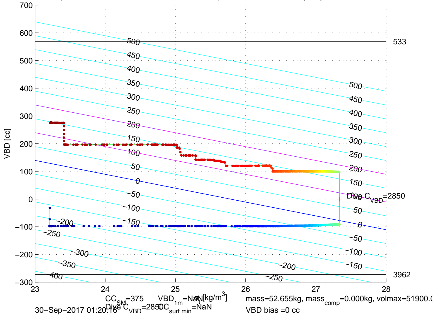
p6350594: SG635 Mission 7 Jul 2017 30-Sep-2017 00:31:59Z – buoyancy contoured
