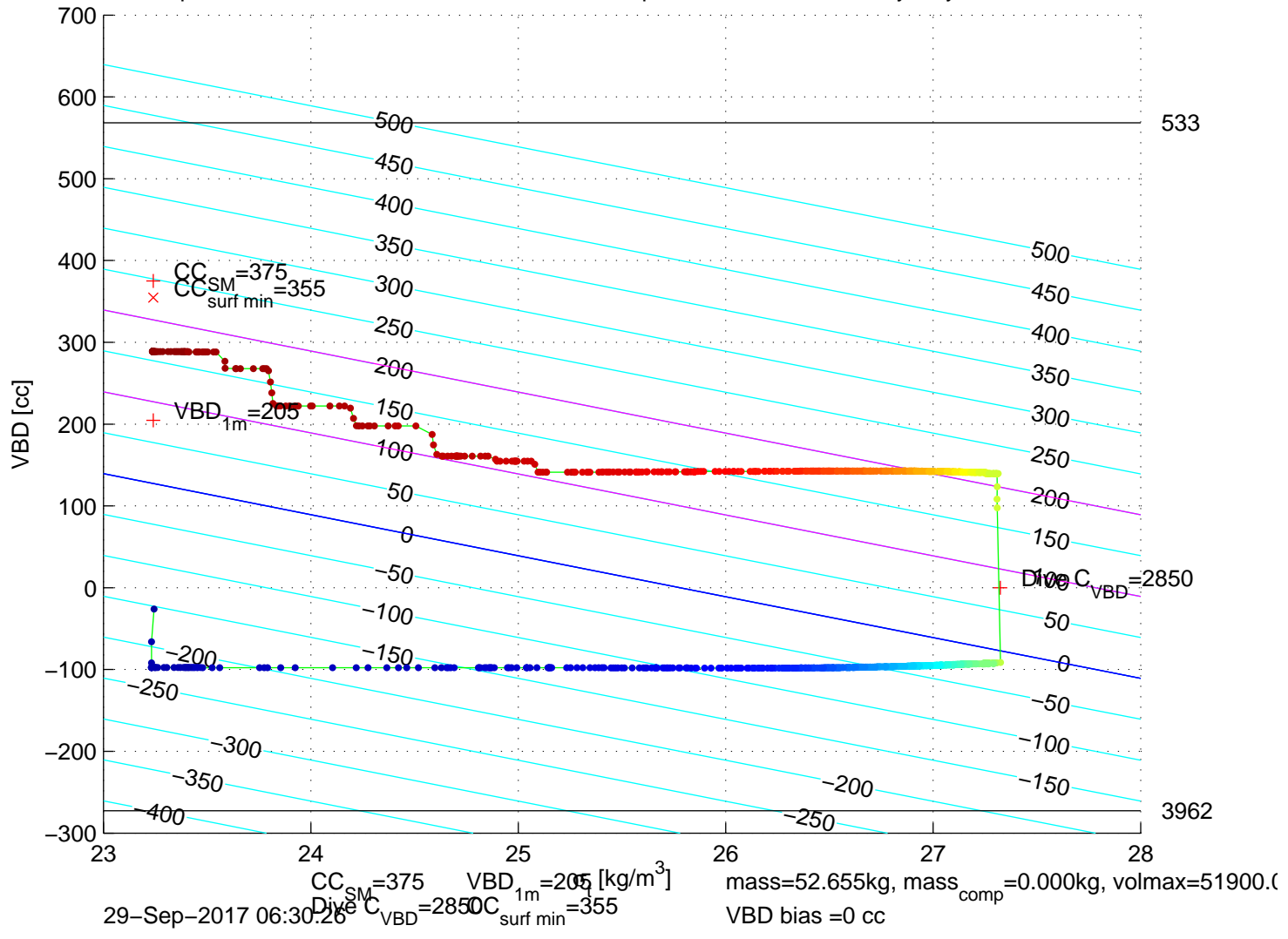
p6350590: SG635 Mission 7 Jul 2017 29-Sep-2017 06:05:47Z – buoyancy contoured
