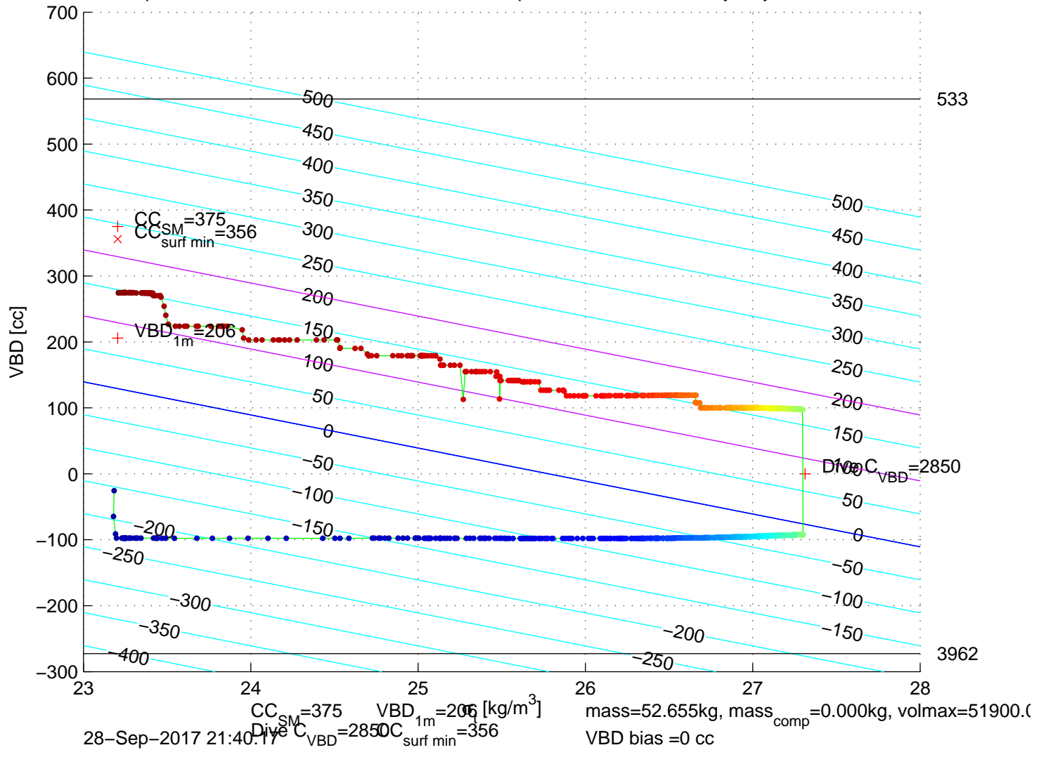
p6350588: SG635 Mission 7 Jul 2017 28-Sep-2017 20:55:15Z – buoyancy contoured
