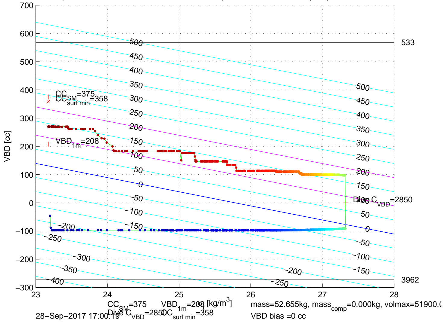
p6350587: SG635 Mission 7 Jul 2017 28-Sep-2017 16:13:48Z – buoyancy contoured
