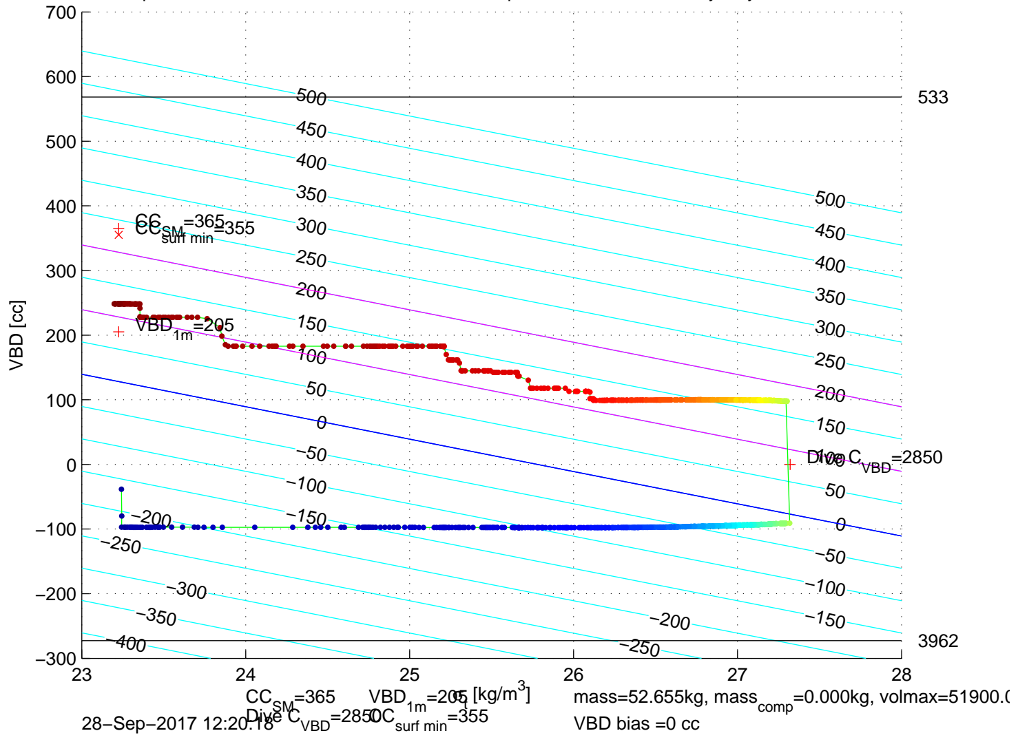
p6350586: SG635 Mission 7 Jul 2017 28-Sep-2017 11:19:49Z - buoyancy contoured
