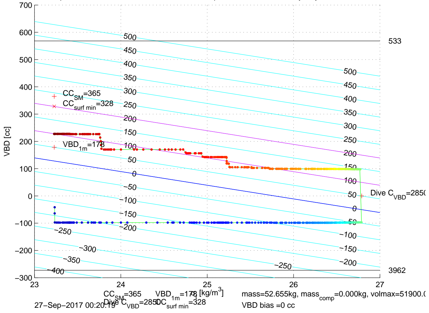
p6350575: SG635 Mission 7 Jul 2017 27-Sep-2017 01:58:56Z – buoyancy contoured
