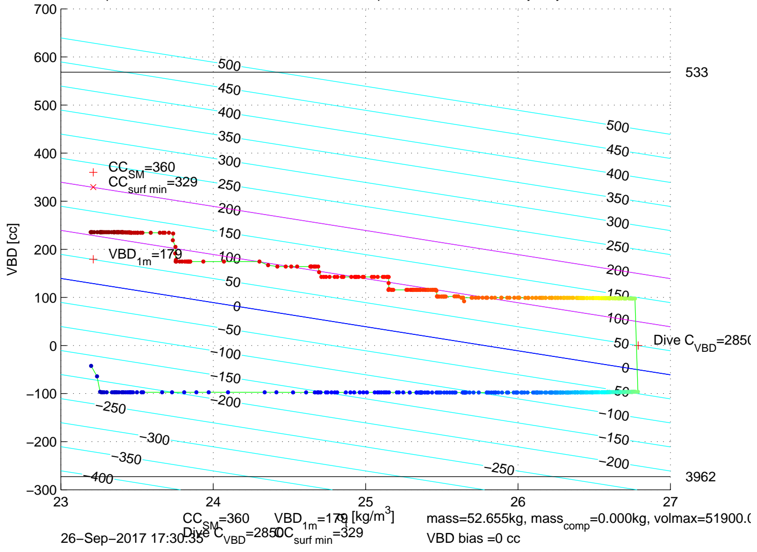
p6350572: SG635 Mission 7 Jul 2017 26-Sep-2017 19:05:56Z - buoyancy contoured
