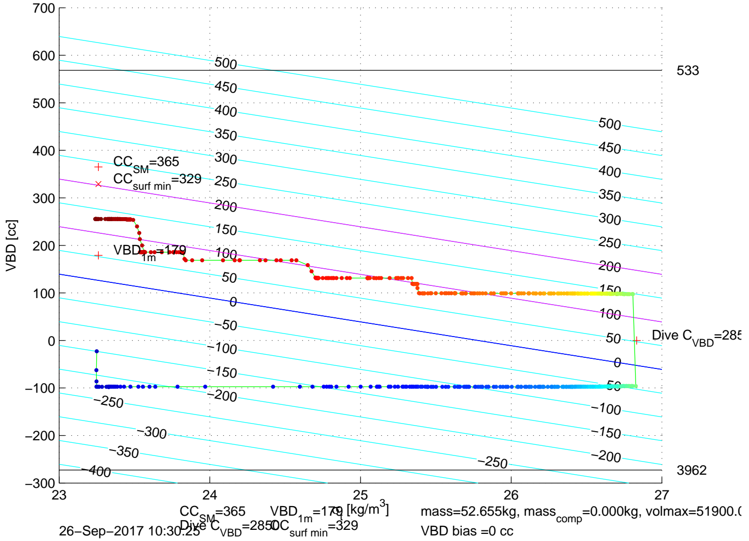
p6350569: SG635 Mission 7 Jul 2017 26-Sep-2017 12:02:46Z – buoyancy contoured
