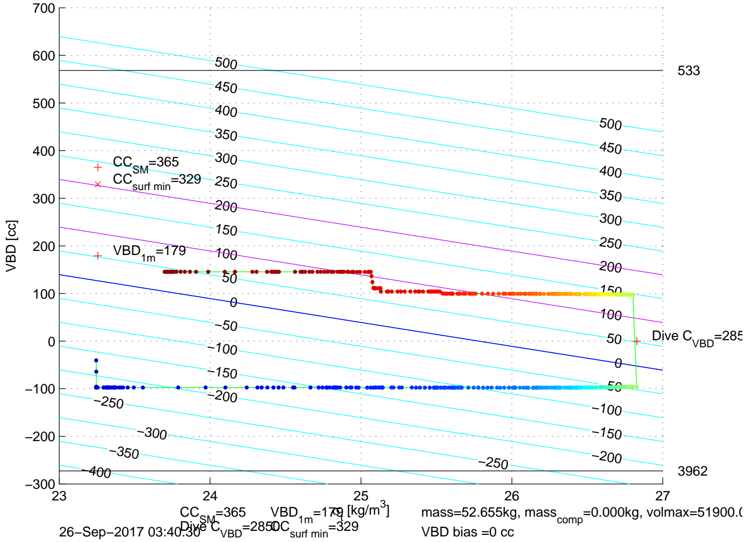
p6350566: SG635 Mission 7 Jul 2017 26-Sep-2017 05:17:37Z – buoyancy contoured
