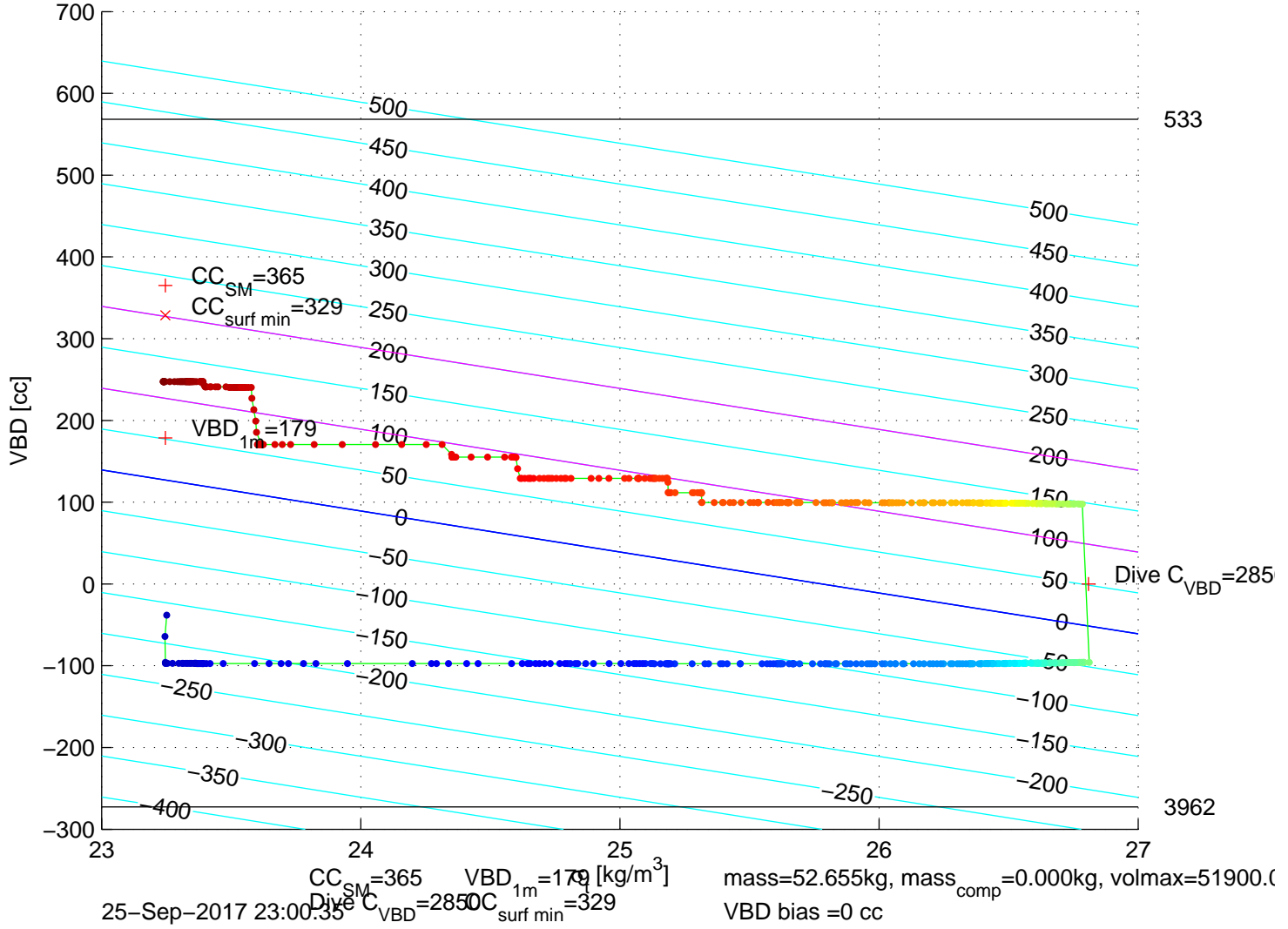
p6350564: SG635 Mission 7 Jul 2017 26-Sep-2017 00:41:02Z – buoyancy contoured
