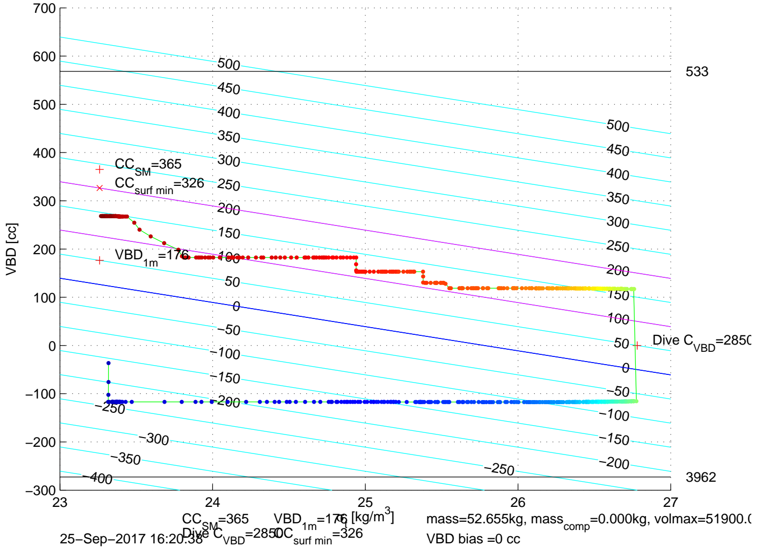
p6350561: SG635 Mission 7 Jul 2017 25-Sep-2017 17:37:52Z – buoyancy contoured
