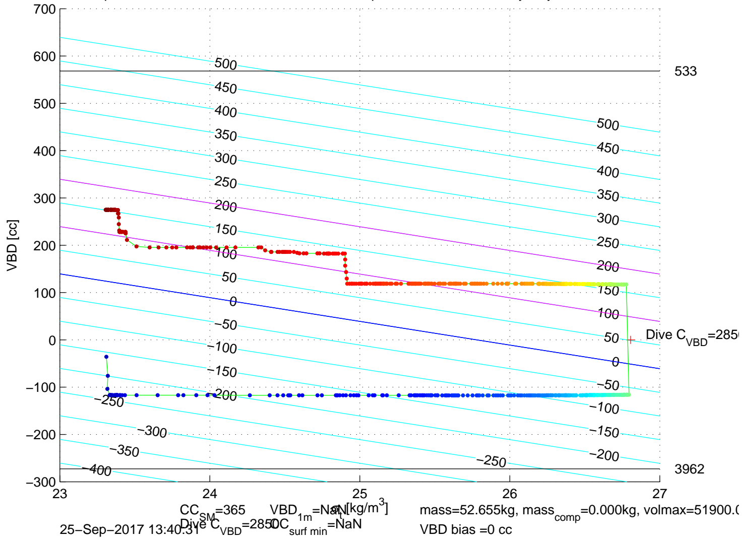
p6350560: SG635 Mission 7 Jul 2017 25-Sep-2017 15:14:35Z – buoyancy contoured
