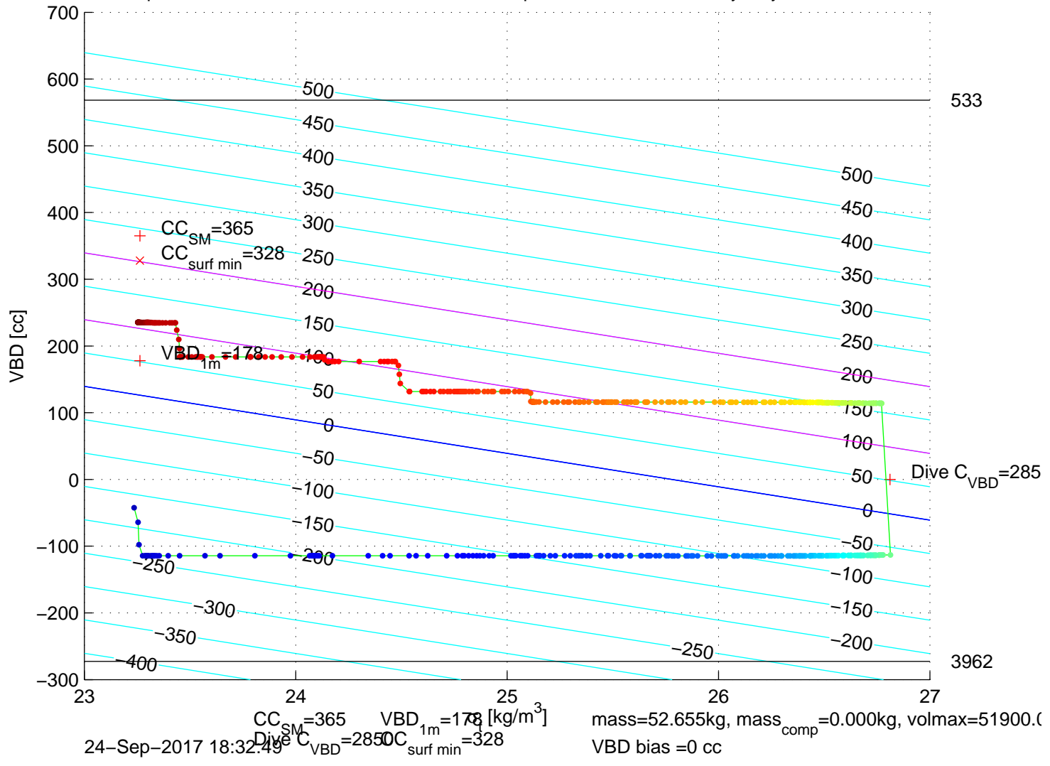
p6350551: SG635 Mission 7 Jul 2017 24-Sep-2017 20:15:16Z – buoyancy contoured
