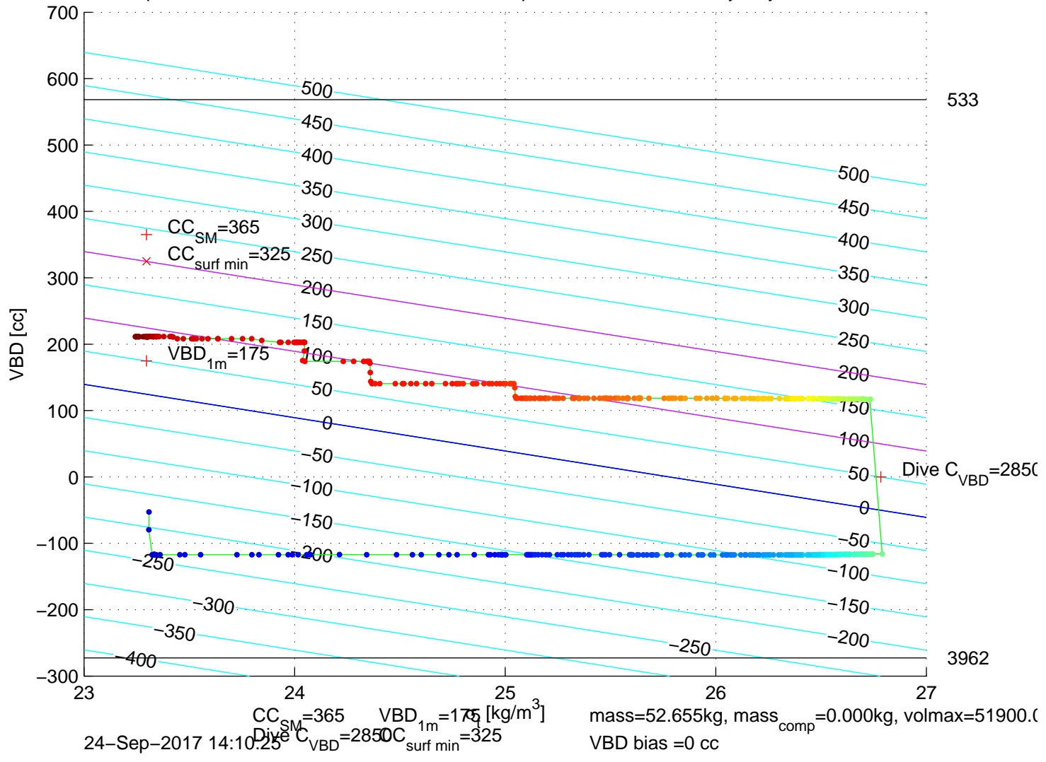
p6350549: SG635 Mission 7 Jul 2017 24-Sep-2017 15:59:57Z – buoyancy contoured
