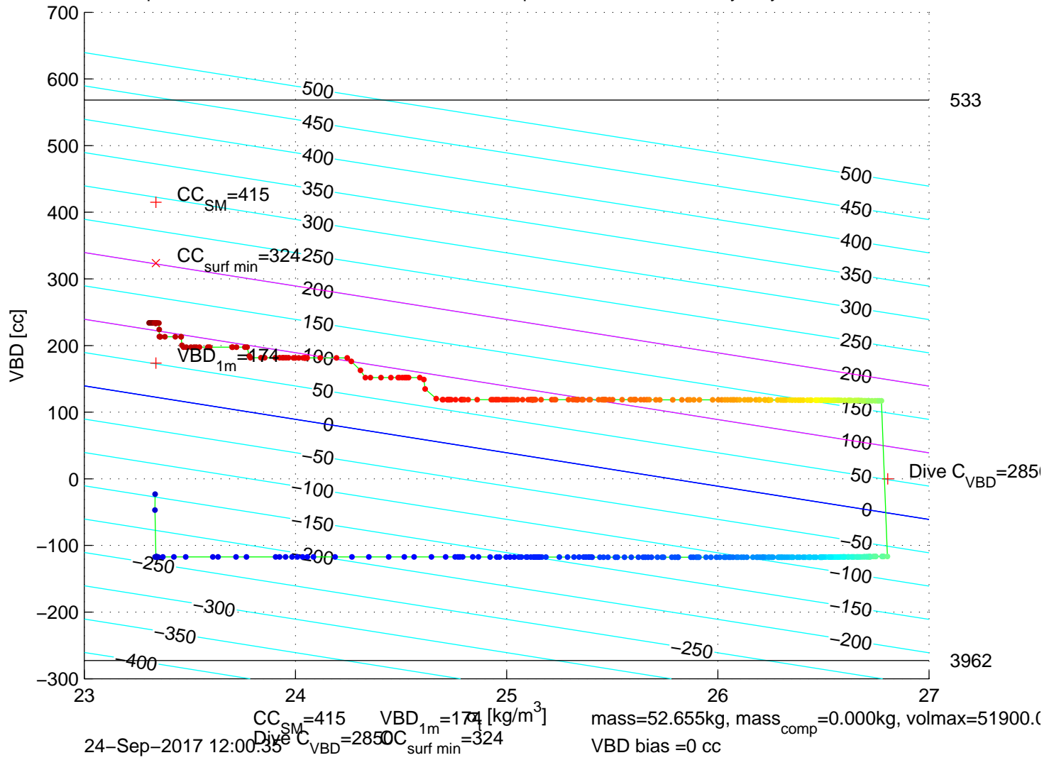
p6350548: SG635 Mission 7 Jul 2017 24-Sep-2017 13:52:56Z – buoyancy contoured
