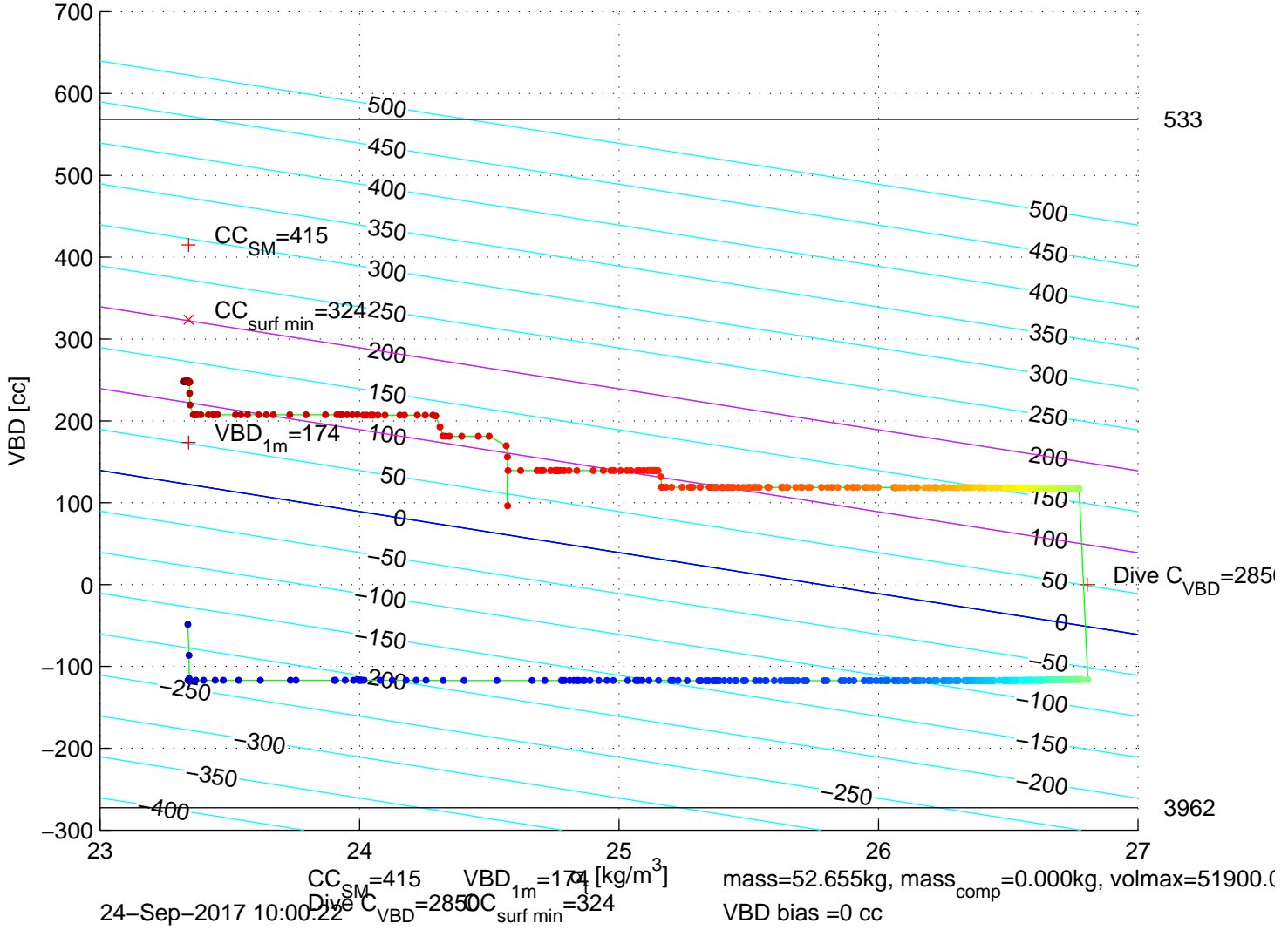
p6350547: SG635 Mission 7 Jul 2017 24-Sep-2017 11:38:32Z – buoyancy contoured
