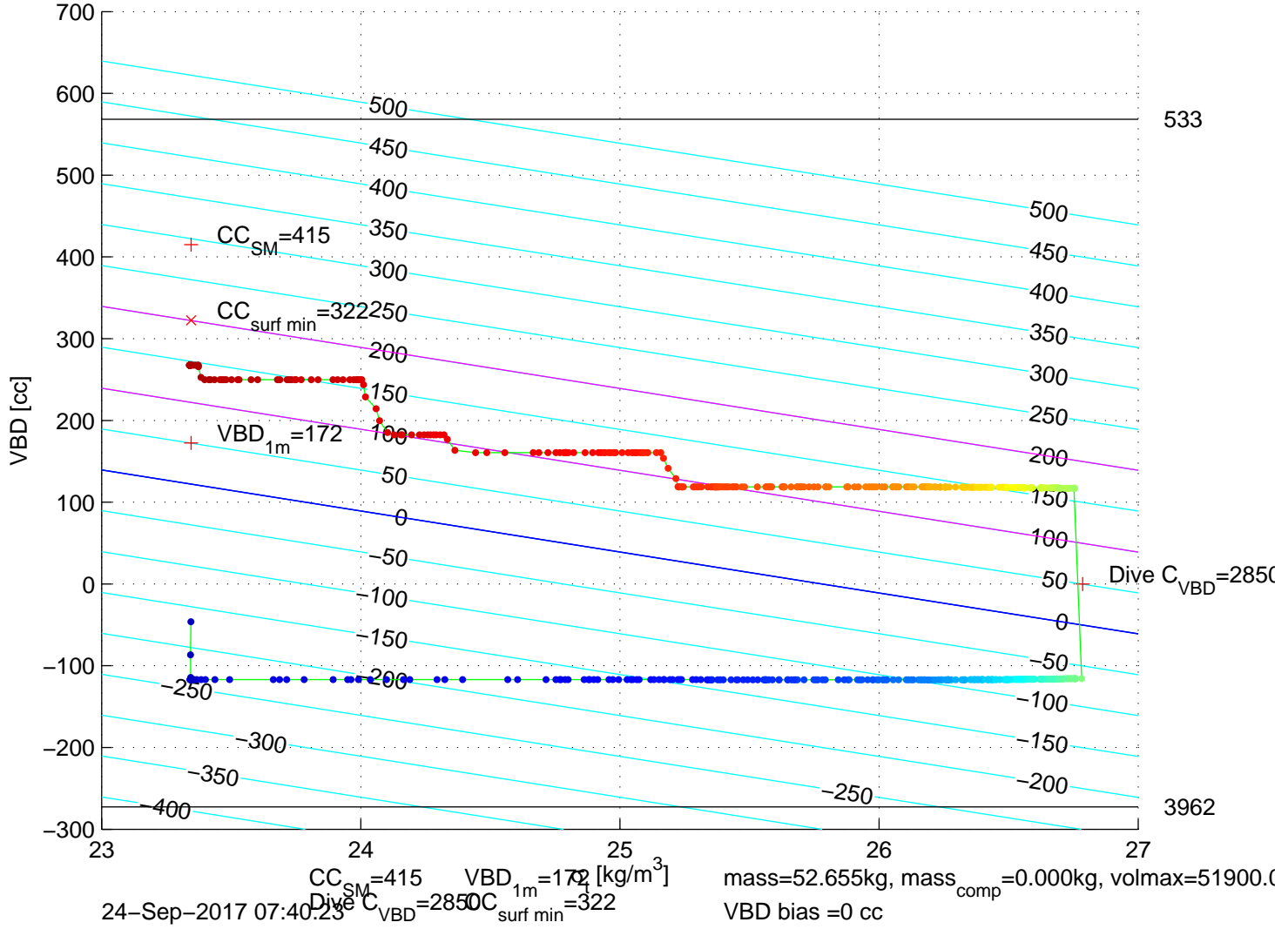
p6350546: SG635 Mission 7 Jul 2017 24-Sep-2017 09:11:54Z – buoyancy contoured
