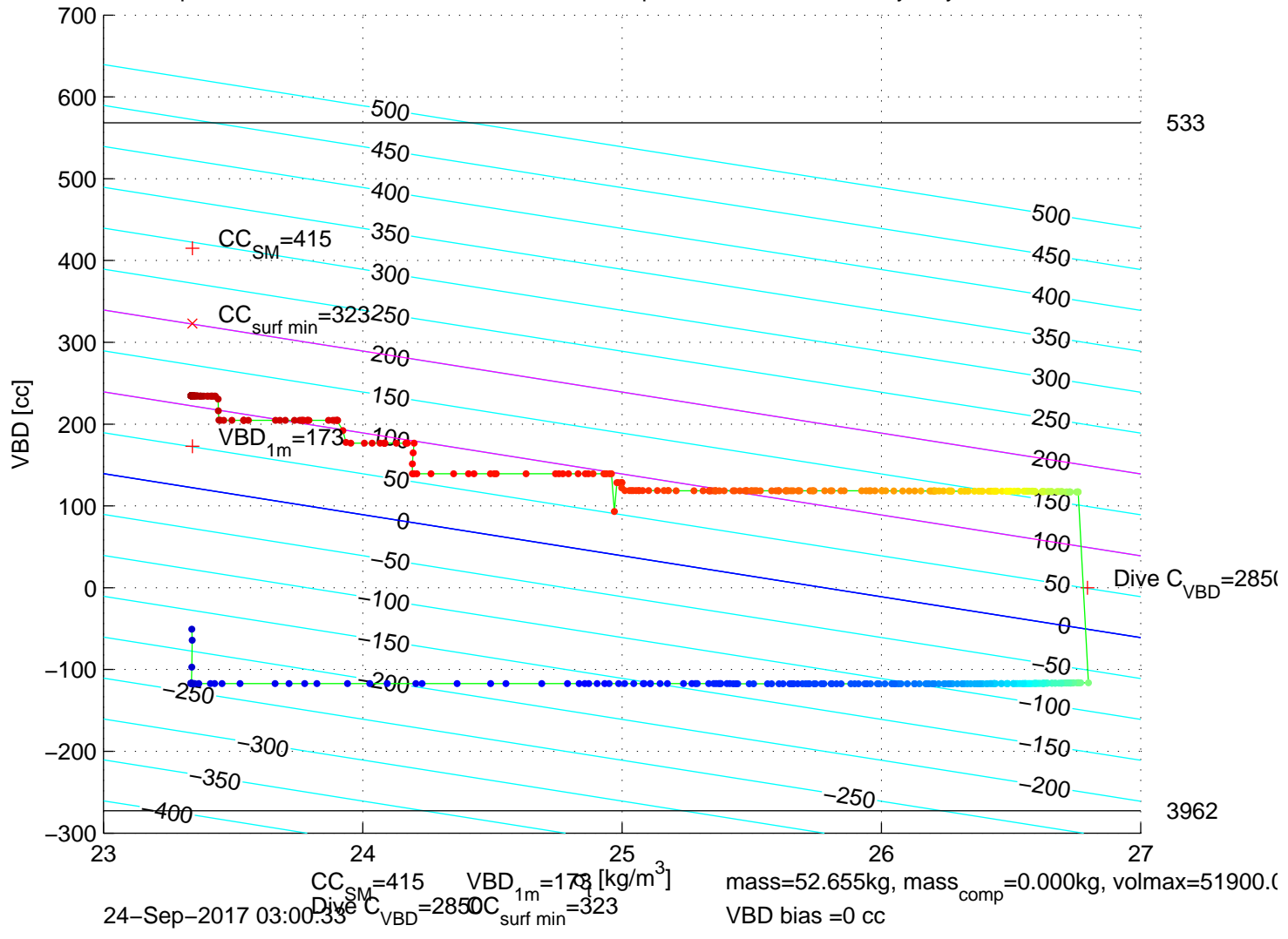
p6350544: SG635 Mission 7 Jul 2017 24-Sep-2017 04:54:47Z - buoyancy contoured
