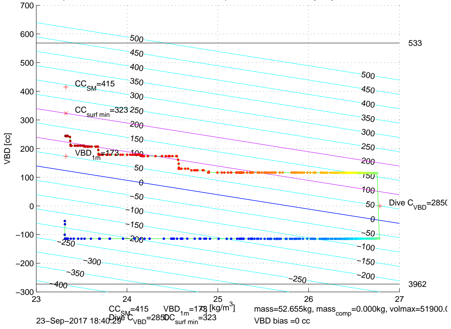
p6350540: SG635 Mission 7 Jul 2017 23-Sep-2017 20:31:53Z – buoyancy contoured
