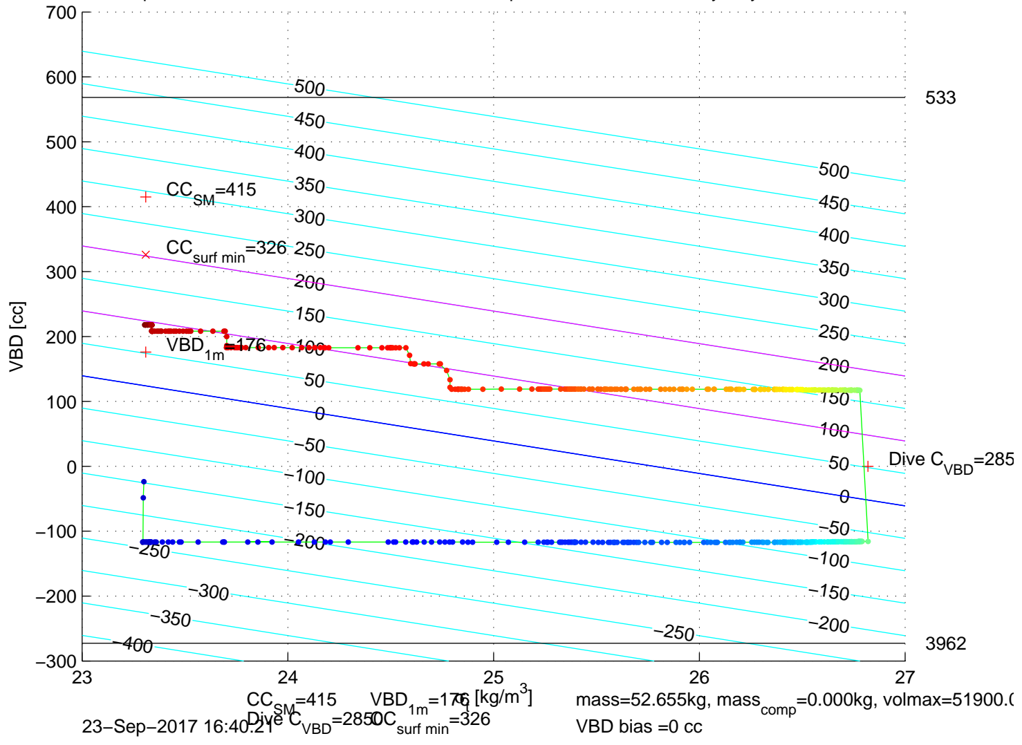
p6350539: SG635 Mission 7 Jul 2017 23-Sep-2017 18:23:23Z – buoyancy contoured
