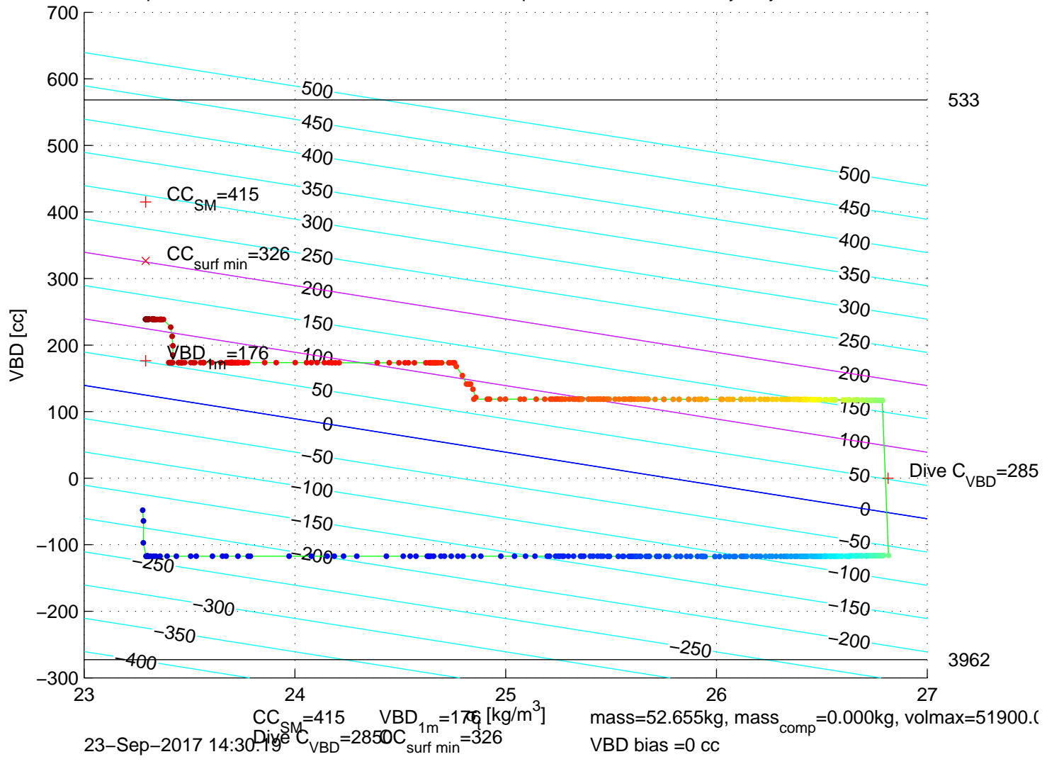
p6350538: SG635 Mission 7 Jul 2017 23-Sep-2017 16:13:50Z – buoyancy contoured
