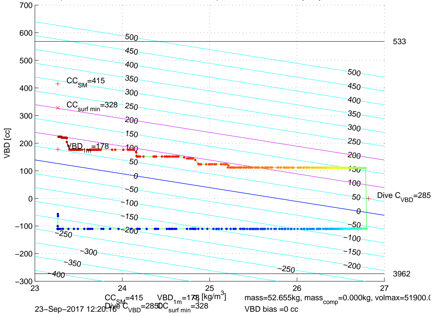
p6350537: SG635 Mission 7 Jul 2017 23-Sep-2017 14:01:31Z – buoyancy contoured
