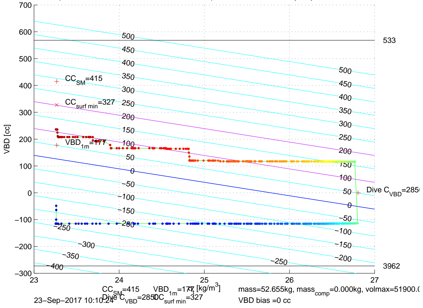
p6350536: SG635 Mission 7 Jul 2017 23-Sep-2017 11:49:16Z – buoyancy contoured
