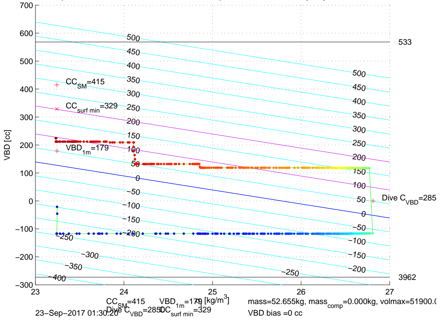
p6350532: SG635 Mission 7 Jul 2017 23-Sep-2017 03:13:50Z – buoyancy contoured
