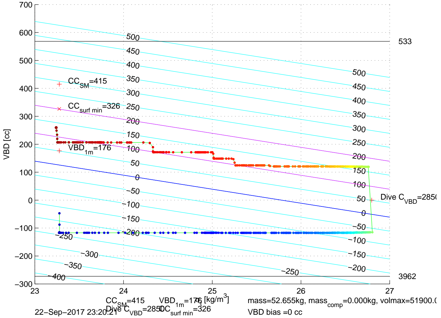
p6350531: SG635 Mission 7 Jul 2017 23-Sep-2017 00:43:18Z – buoyancy contoured
